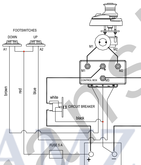
WIRING DIAGRAM - 2 TERMINALS ELECTRIC MOTOR
