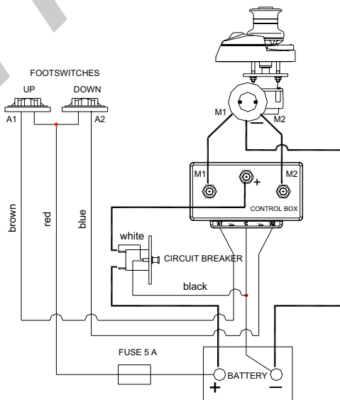
WIRING DIAGRAM - 3 TERMINALS ELECTRIC MOTOR
